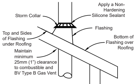
FIG. 15 - Flashing Installation
