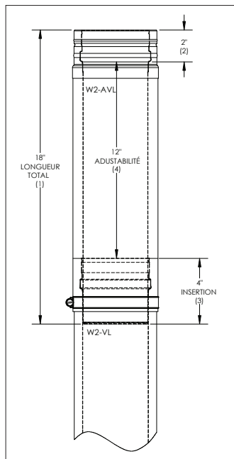
Figure 1a (paroi double)
