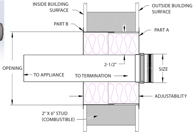
Figure 4 Single Wall Thimble Installation
