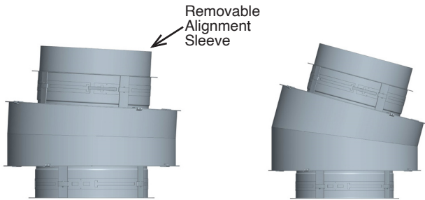
Figure 35a: 3° Elbow
