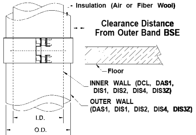
Figure 1 - Detail of Clearance Distance
