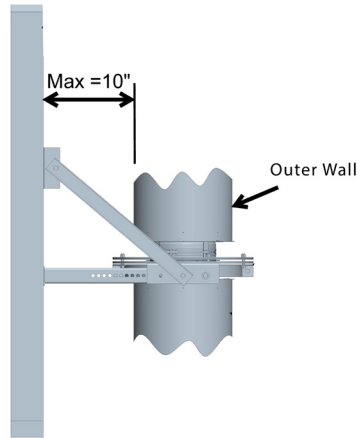
Figure 47c - Maximum Adjustment
