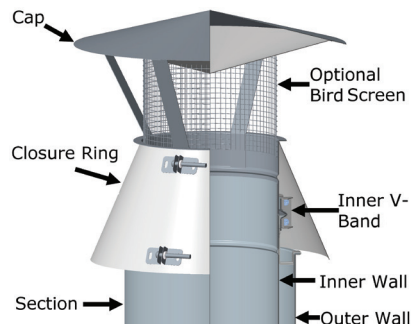
Figure 68 - Rain Cap (RC) installed
