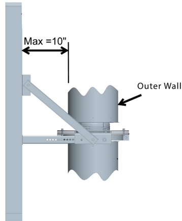
Figure 47c - Maximum Adjustment
