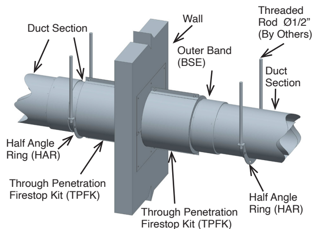
Figure 108: Supports for duct through fire-rated wall (DIS3Z only)
