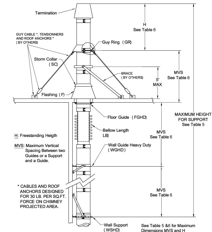
Figure 3 - Maximum Supported Height
