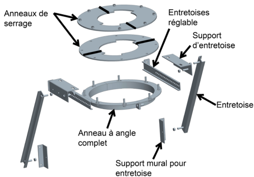
Schéma 47a- Support mural (WSHD)
