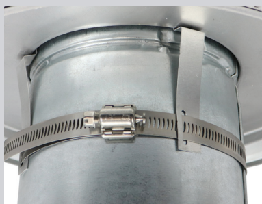
Adjustable Worm Gear Clamp
