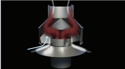
When wind enters from the bottom, flue gases flow up and out of the DIKAPT.
