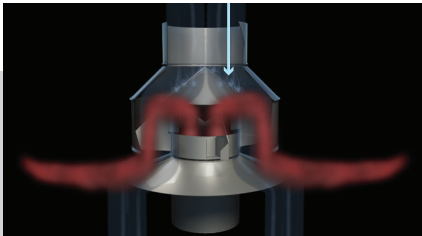
As rain enters from the top, DIKAPT diverts water and allows flue gases to exit.
