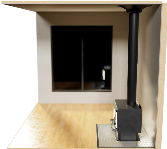
STRAIGHT-UP INSTALLATION
