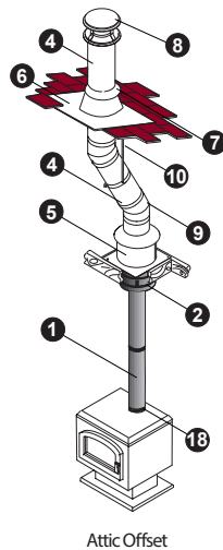
Attic Offset
