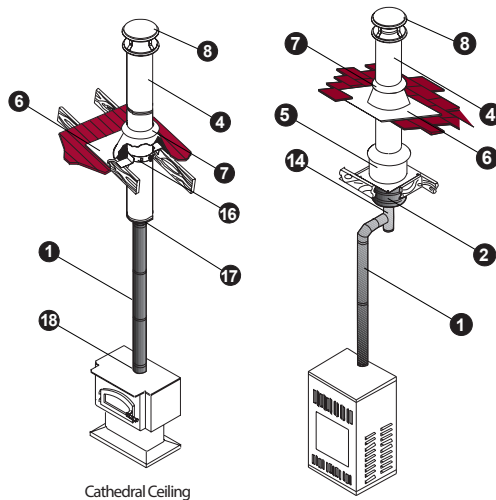
Cathedral Ceiling
